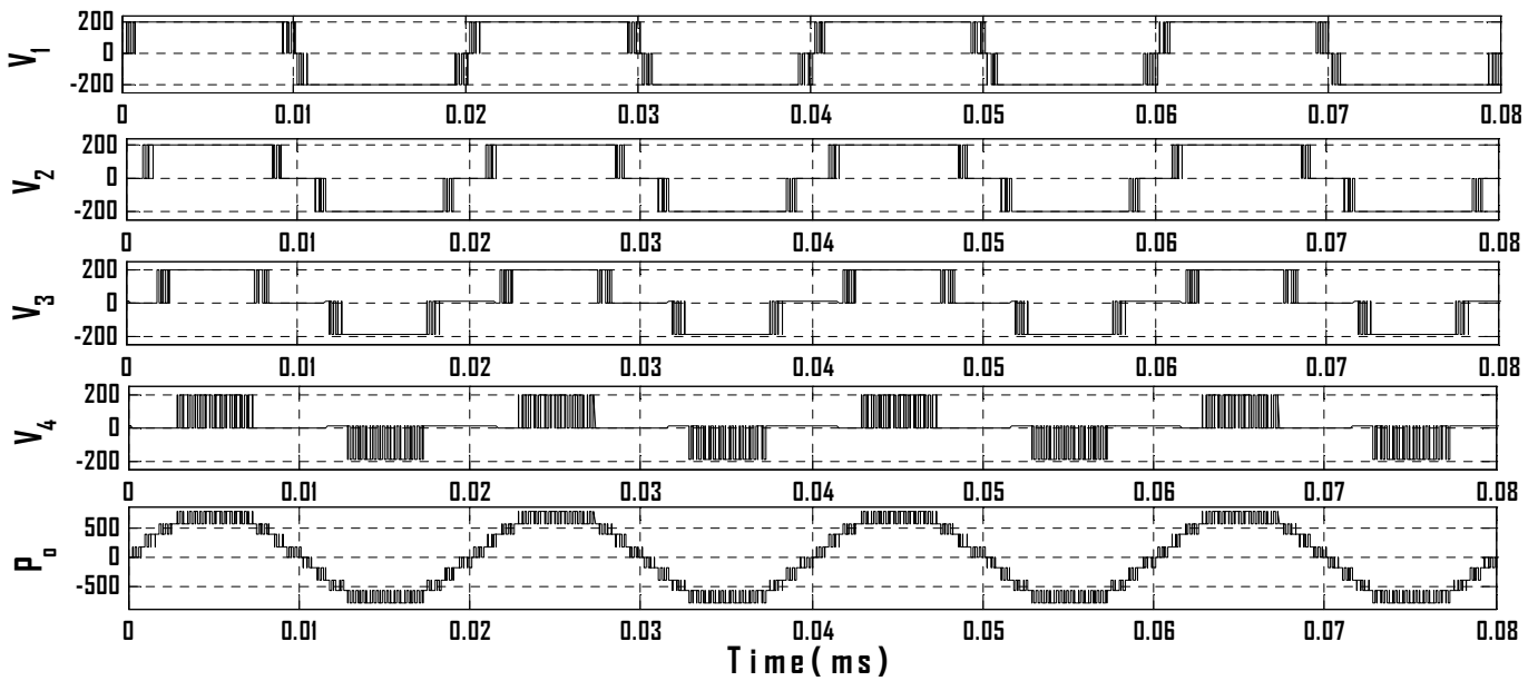
Figure 2: Voltage profile for the 9-level CHB inverter with the conventional design
