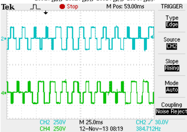
Figure 10: Experimental module voltages.
