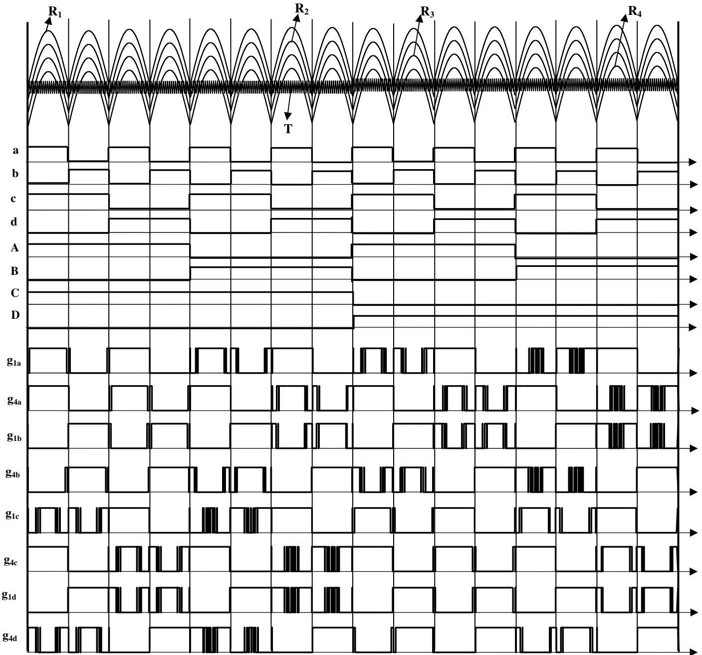
Figure. 5: Switching patterns of the proposed modulation strategy.
