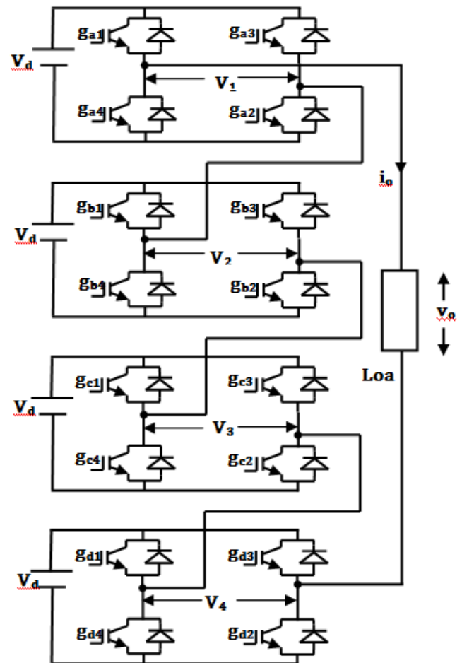
Figure 1: Configuration of 9-level cascade H-bridge multilevel inverter.
