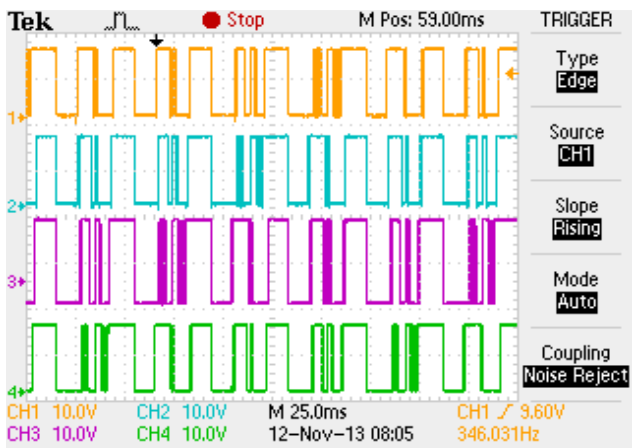
Figure 9: Experimental Gate signals.
