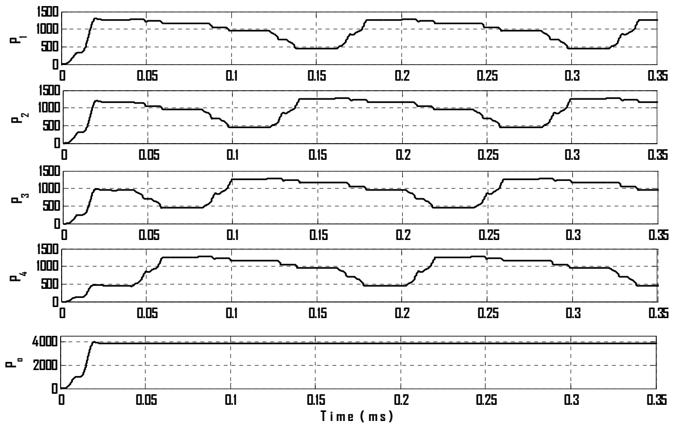
Figure 7: Power profile of CHB inverter under the proposed control strategy
