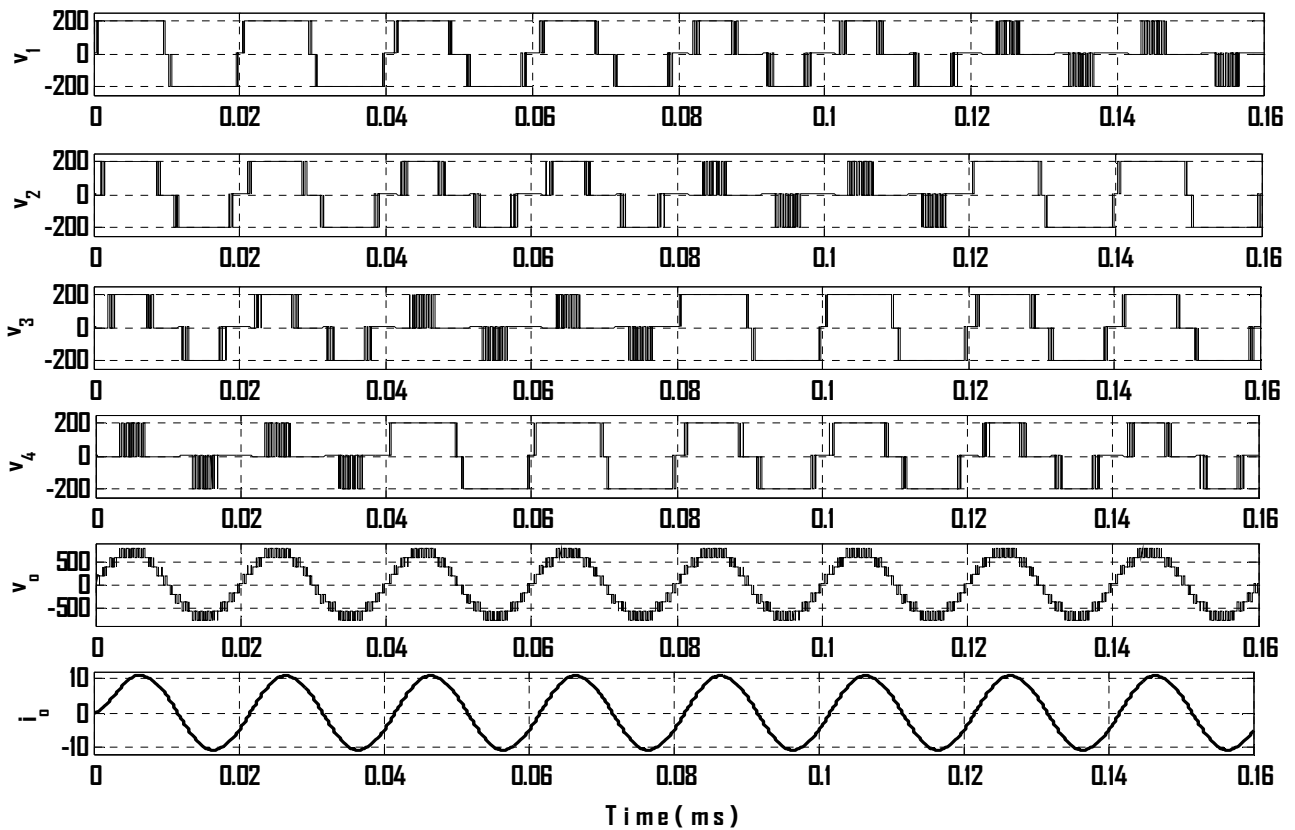
Figure 6: Simulated output voltages and load current
