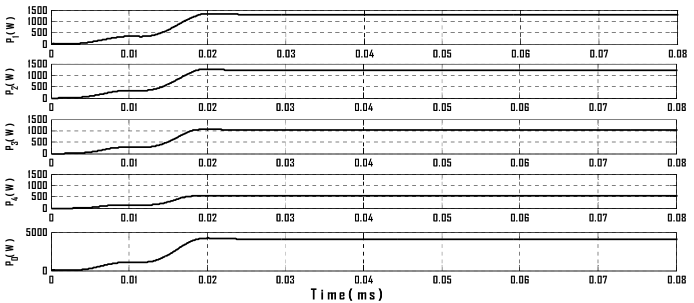
Figure 3: Power profile of the 9-level CHB inverter under the conventional control method
