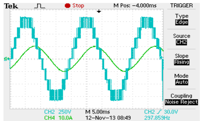
Figure 11: Experimental waveforms of the output voltage and load current
