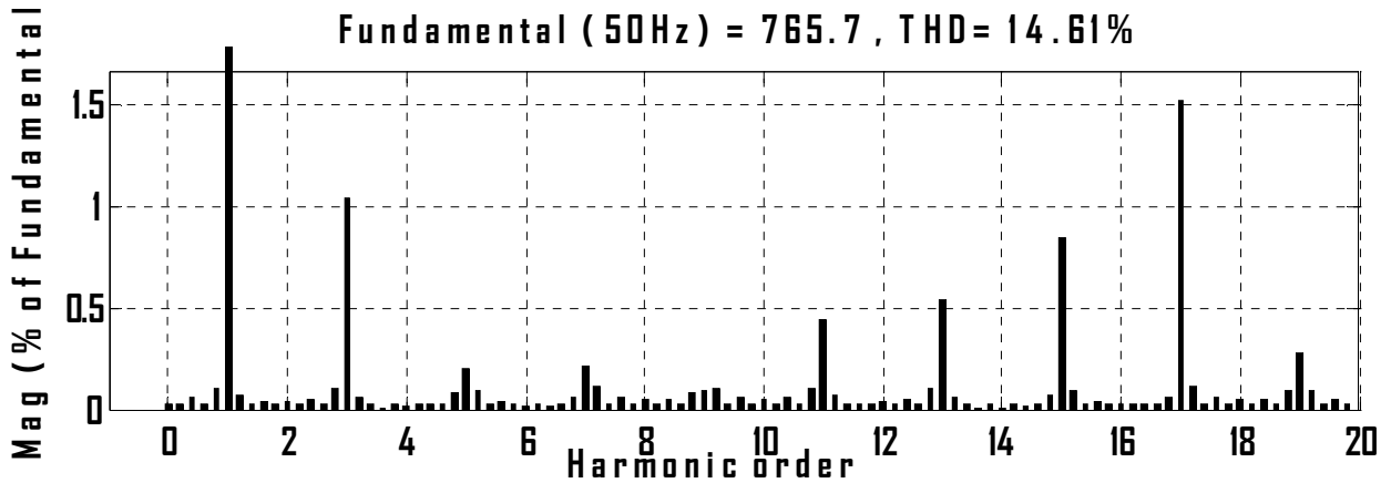
Figure 8: Harmonic profile of the CHB inverter output voltage.
