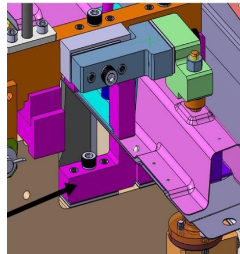
Figure 2: Experimental set up (machine) and schematic of the resting block
