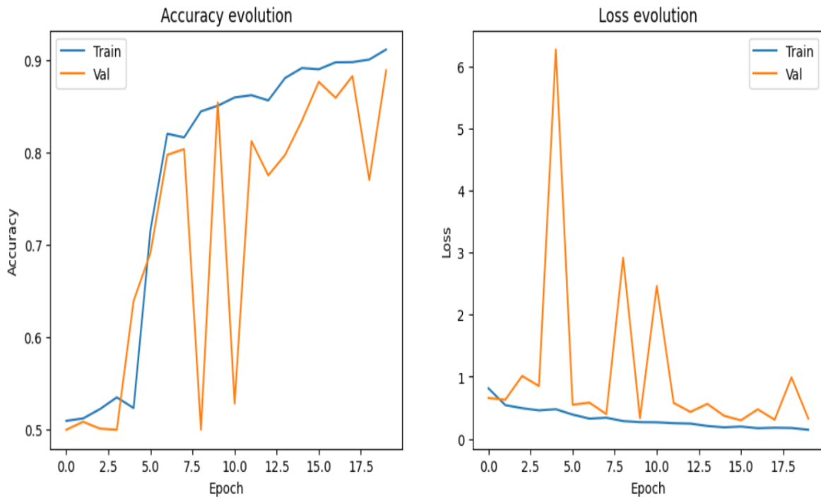
Figure 3: Training accuracy and loss in VGG model
