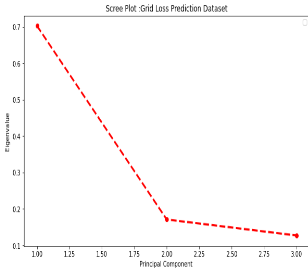
Figure 3: Eigenvalue representation for grid loss prediction dataset
