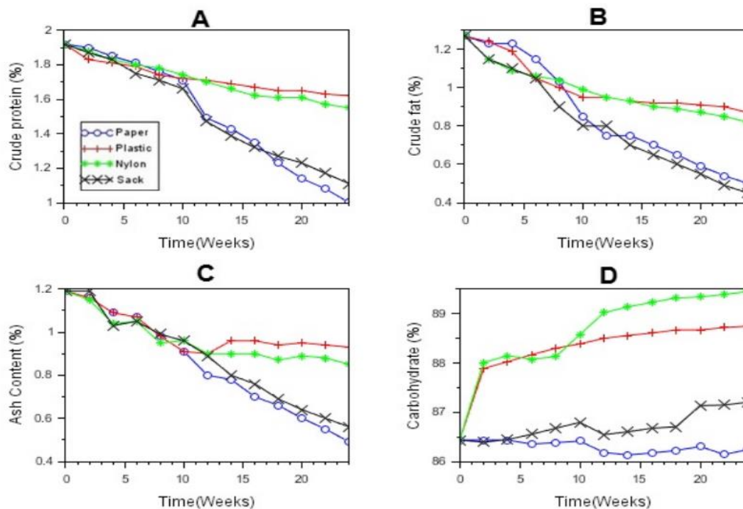
Figure 3: Variation in crude protein (A), crude fat (B), ash content (C) and carbohydrate (D) against storage time
