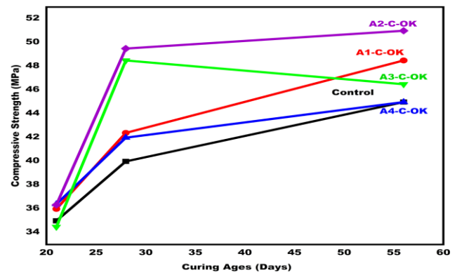
Figure 12: Mortar Strength of calcined Owode-Ketu blended cement
