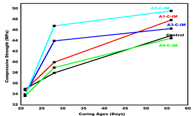
Figure 13: Mortar strength of calcined Imotoyewa blended cement
