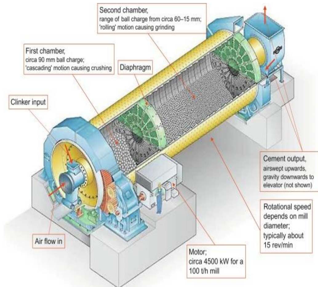
Figure 1: Overview of horizontal or ball mill [21]
