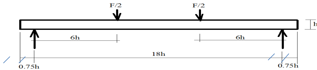
Figure 1: Four-point bending test set-up [20].
